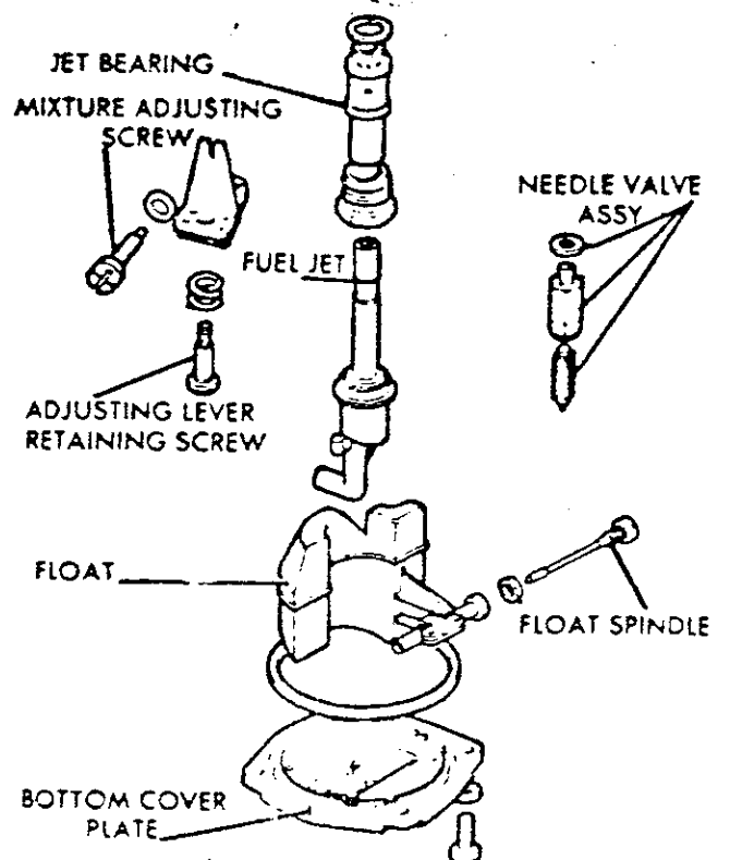
S.U. HIF CARBURETOR DISASSEMBLY
