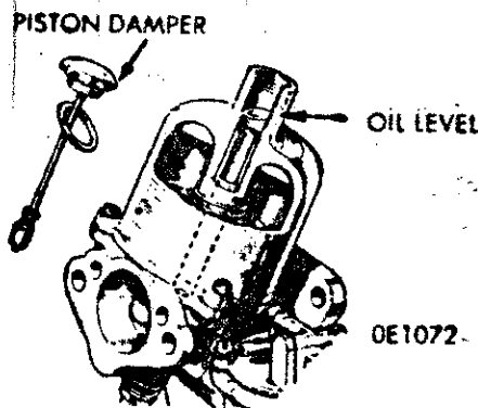
CARBURETOR LUBRICATION
