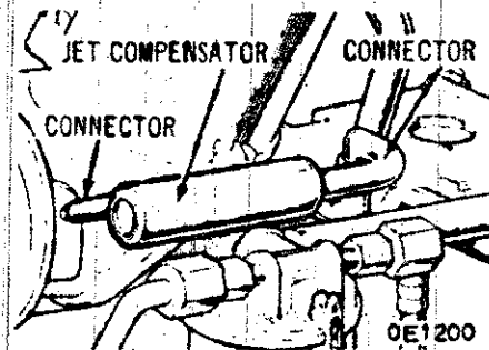
JET COMPENSATOR - TYPE II
