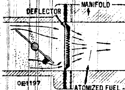
FUEL DEFLECTOR
