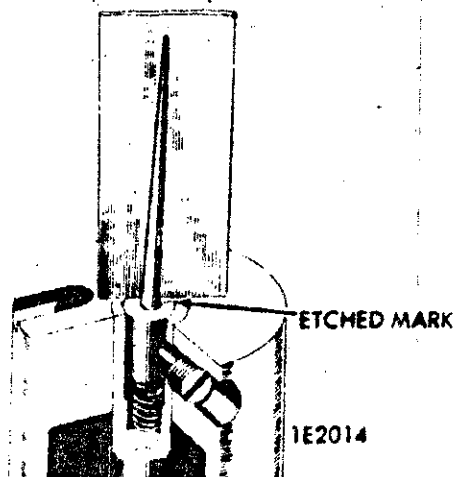
METERING NEEDLE ADJUSTMENT
