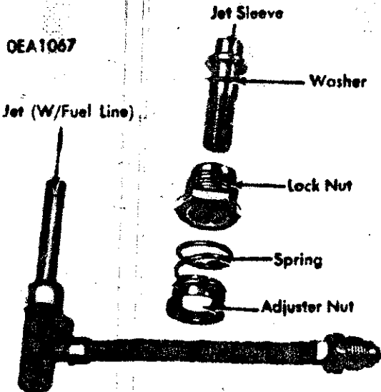
JET DISASSEMBLY (LATE MODELS)
