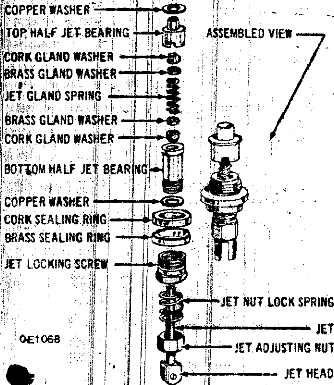
EXPLODED VIEW OF JET (EARLY MODELS)
