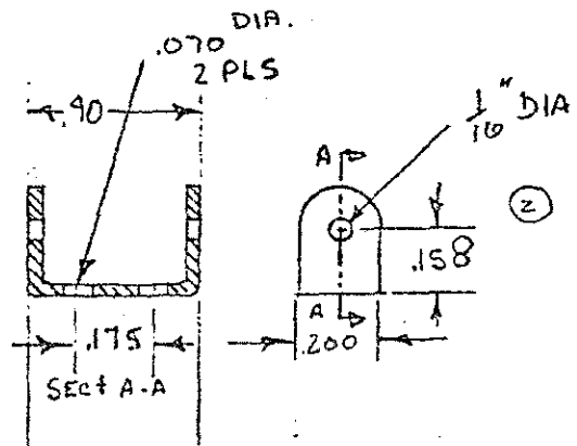
② PIN M.DOC 1013-0 U-BRACKET
