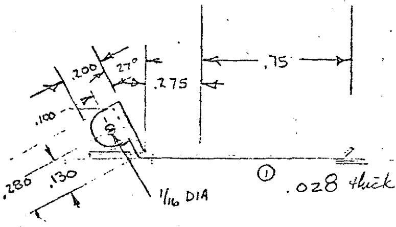
① PIN M.DOC 1012-0 FLAP.
