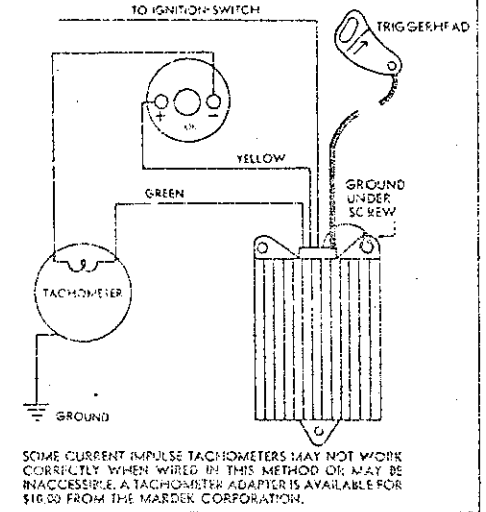
HOW TO REWIRE YOUR CURRENT IMPULSE TYPE TACHOMETER WITH THE MOBELEC Fig. 6B
