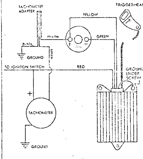
HOW TO INSTALL THE VOLTAGE IMPULSE TACHOMETER ADAPTER Fig. 5B
